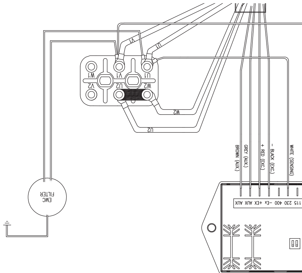
WIRING DIAGRAM OF SK160 1 PHASE
